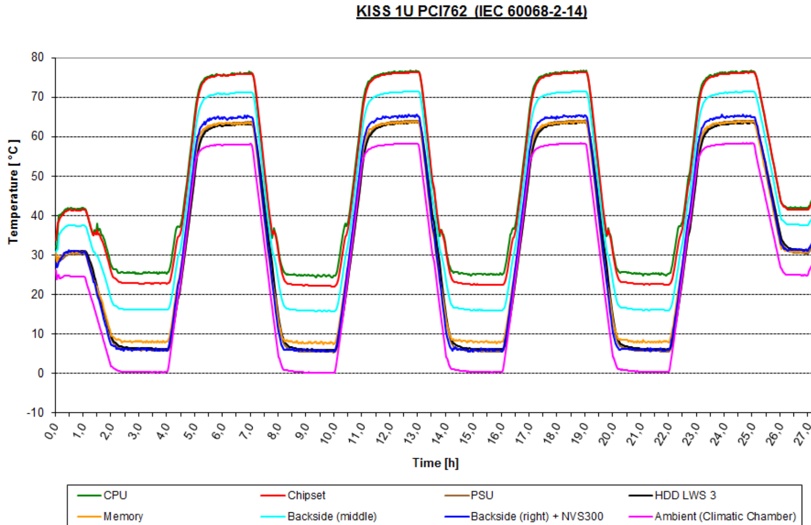
Fig. 7 Measurement diagram: Change of temperature, operating
