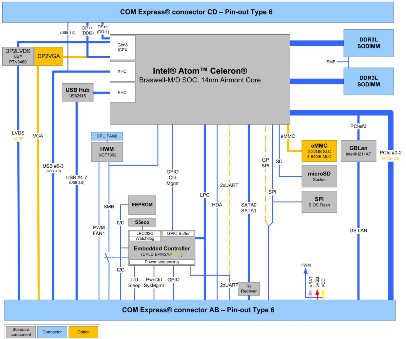
Figure 1: Block Diagram of COMe-cBW6
