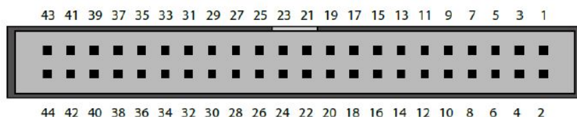
Figure 15: GPIO Internal Connector
