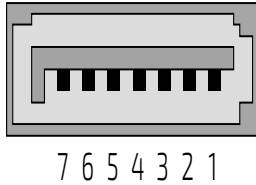
Figure 20: SATA Connector
