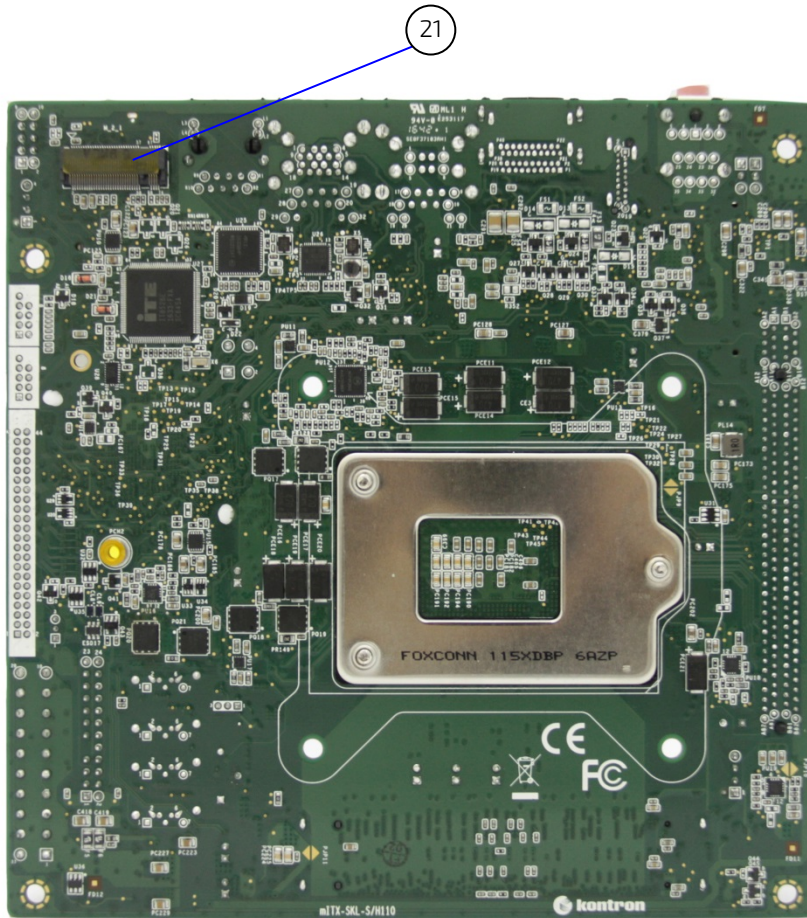
Figure 4: Bottom Side
