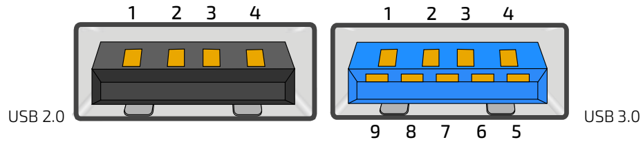
Figure 6: USB 2.0 / 3.0 socket
