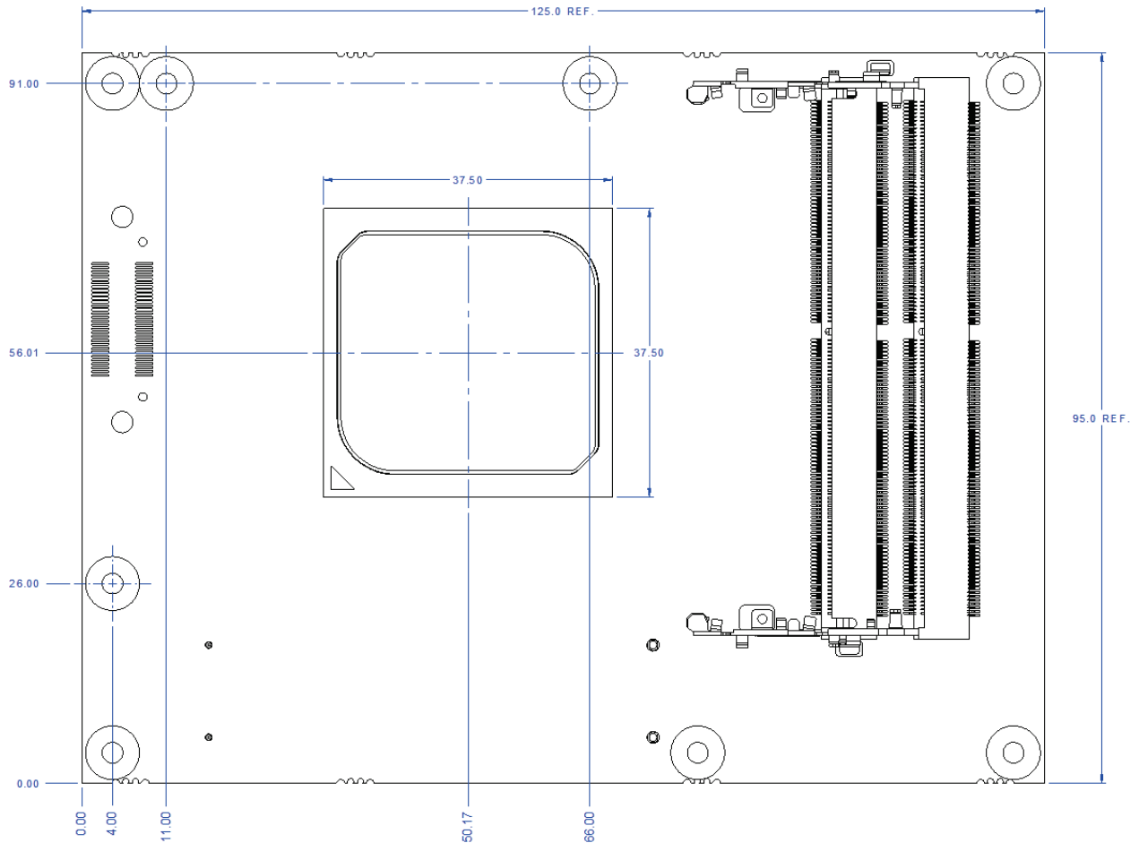
Figure 7: Module Dimensions
