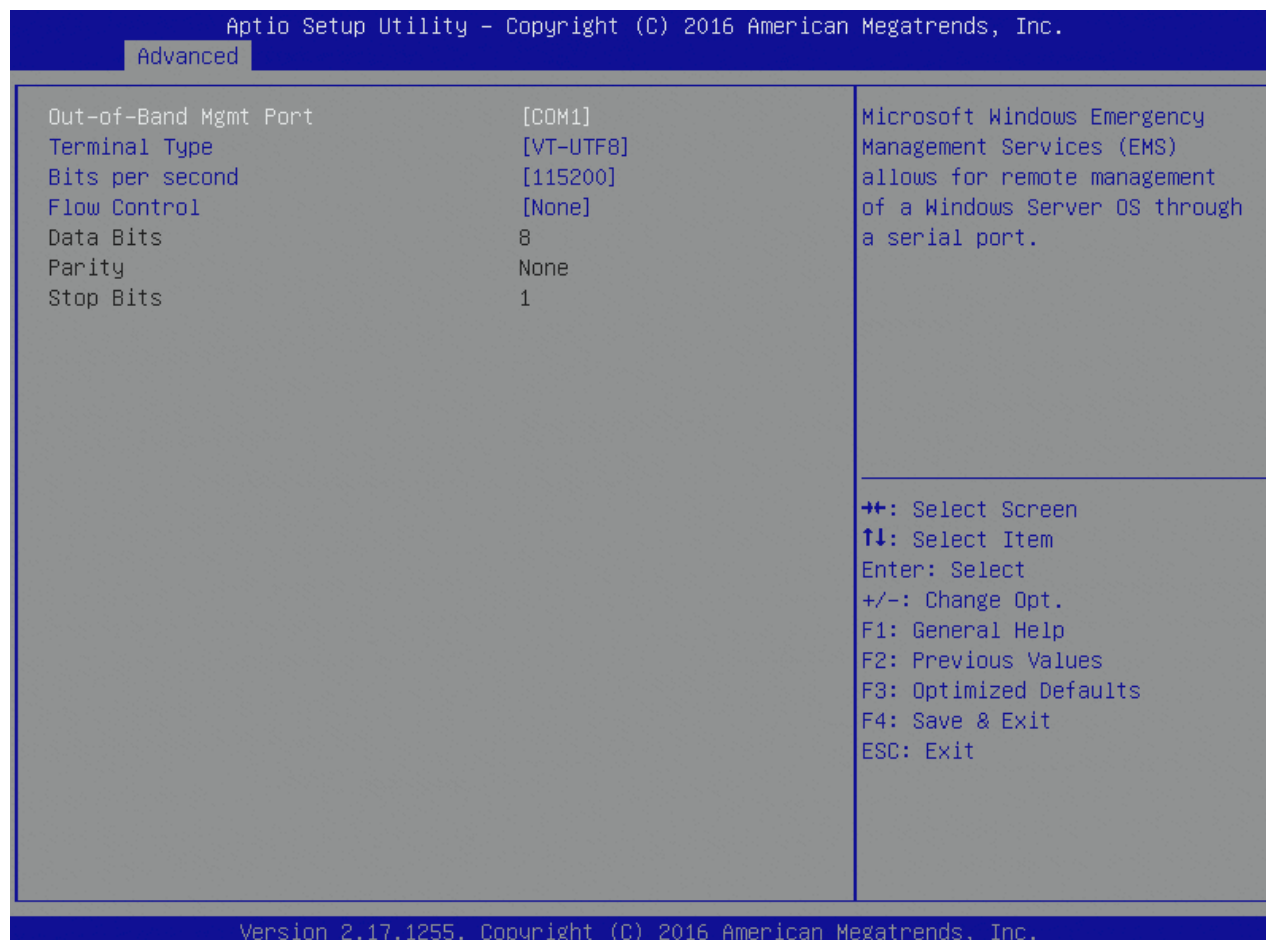
Figure 34: Out-of-Band Management Console Redirection Settings Menu Screen
