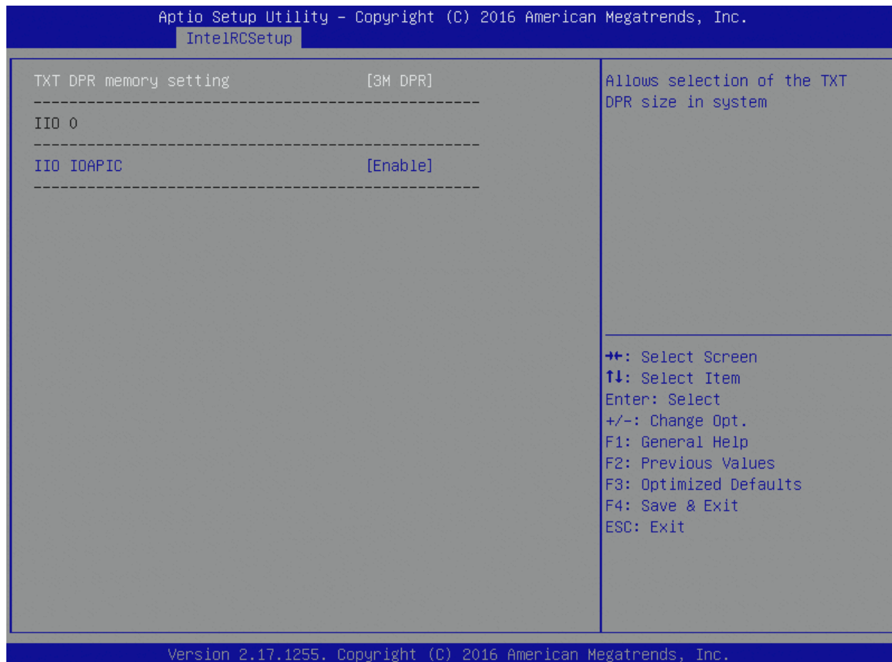
Figure 84: IIO General Configuration Menu Screen
