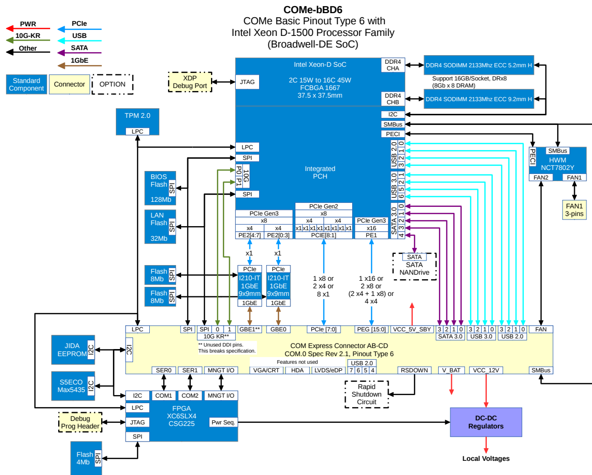
Figure 1: Block Diagram COME-bBD6
