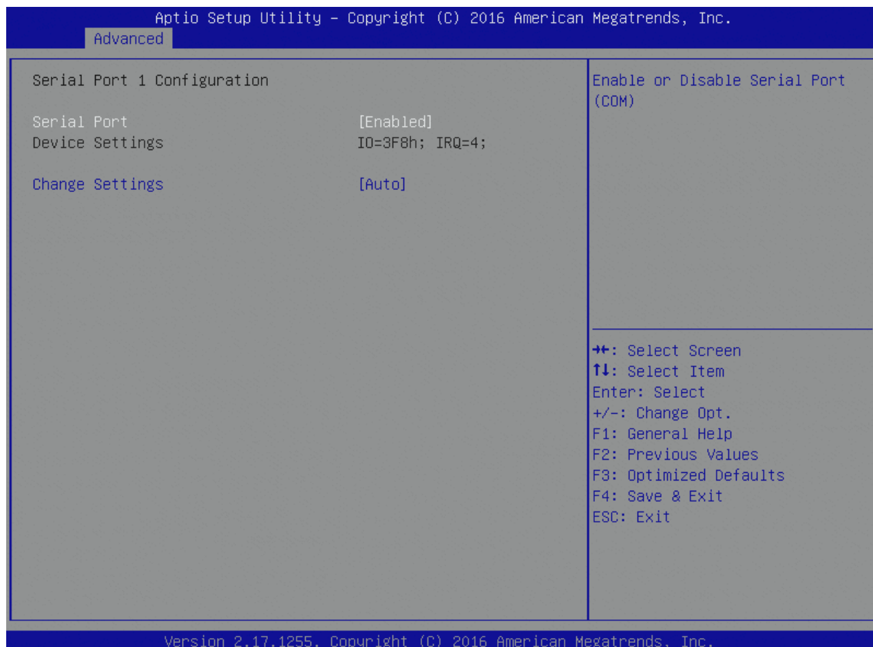
Figure 24: FPD UART Serial Port 1 Configuration Menu Screen
