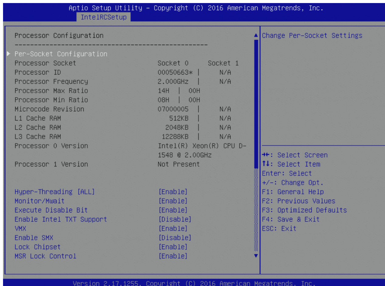
Figure 44: Processor Configuration Menu Screen
