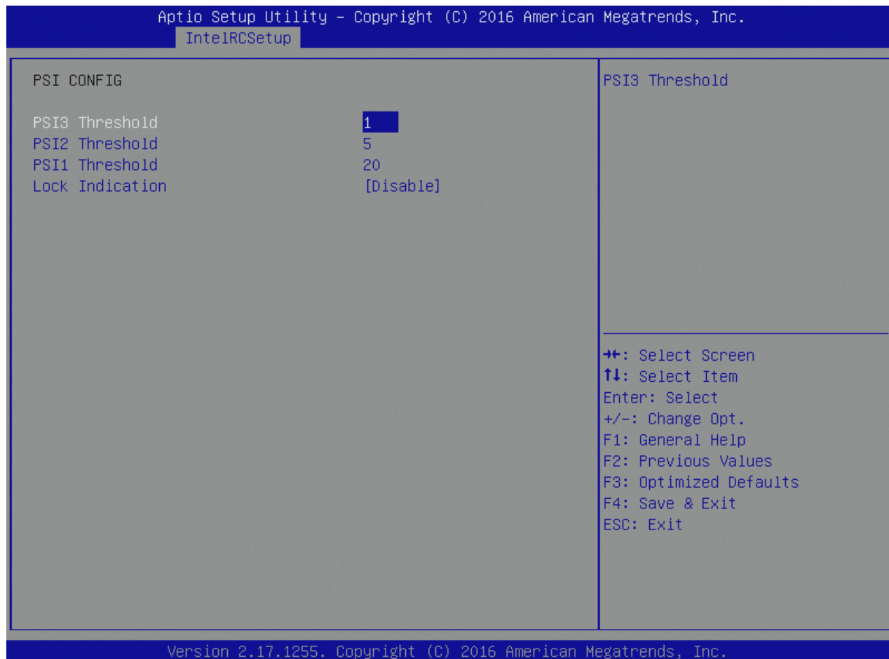
Figure 58: PSI Config Menu Screen
