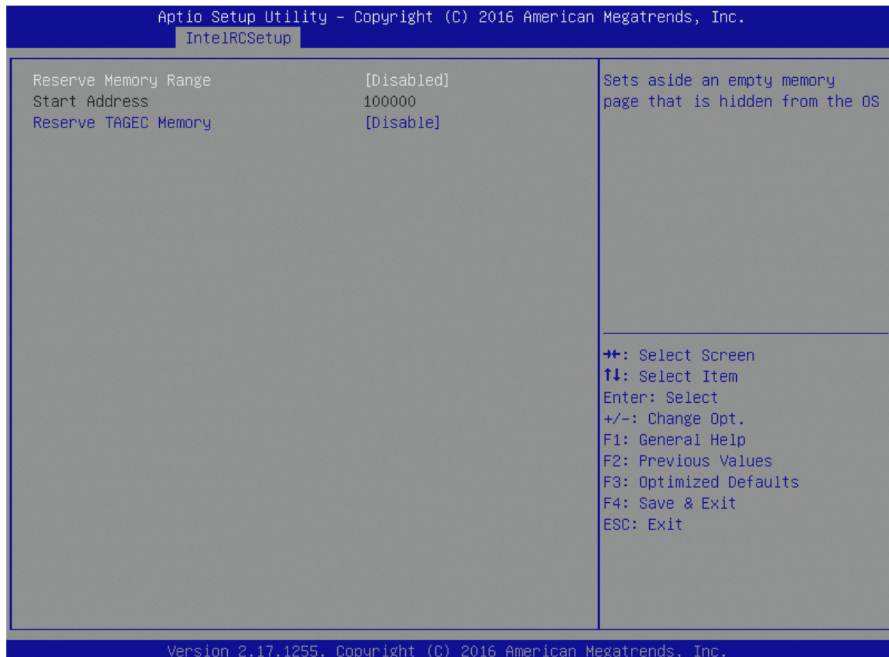
Figure 110: Reserved Memory Menu Screen
