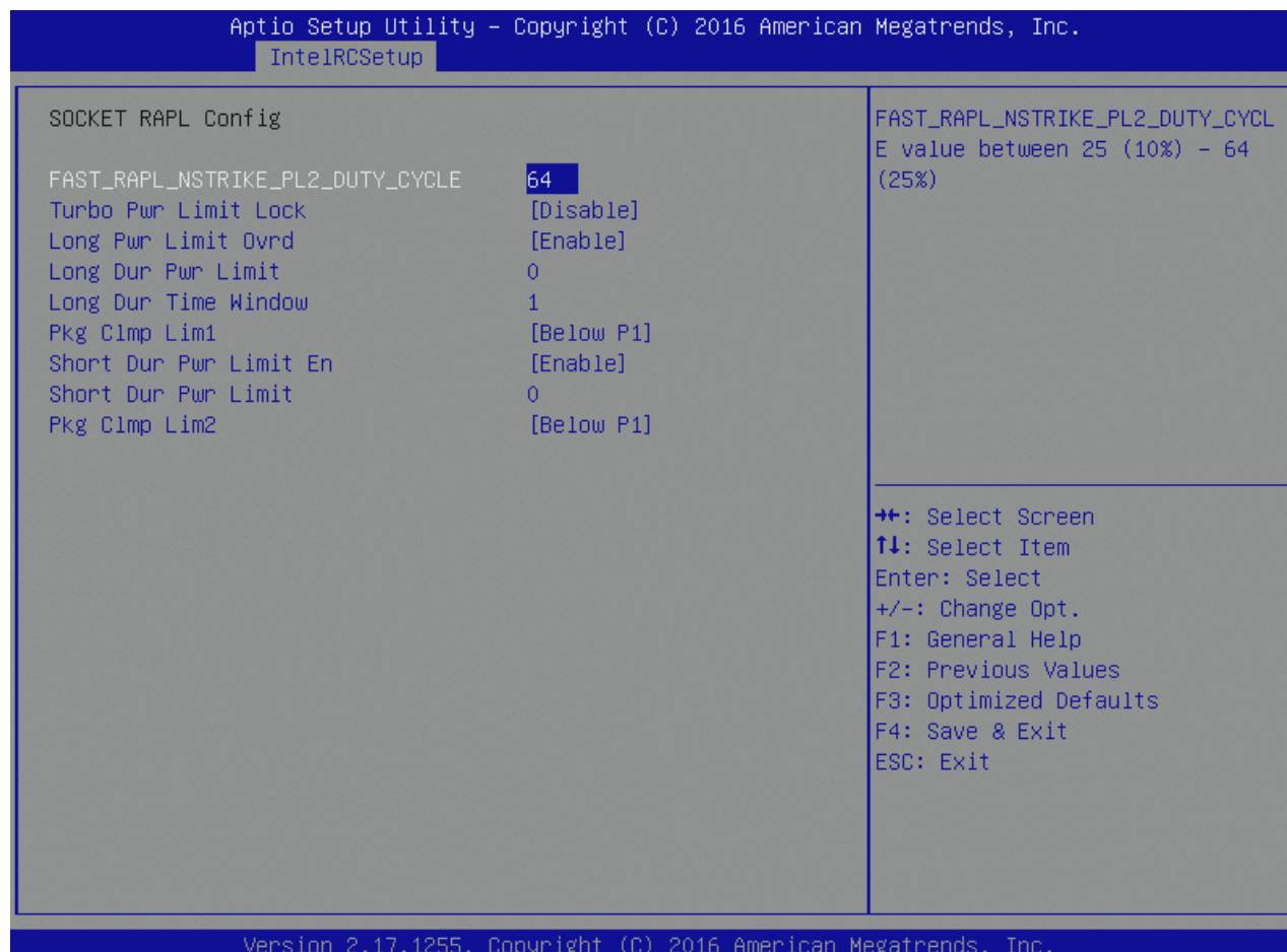
Figure 65: Socket RAPL Config Menu Screen
