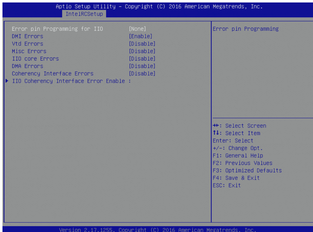
Figure 107: IIO Error Enable Menu Screen
