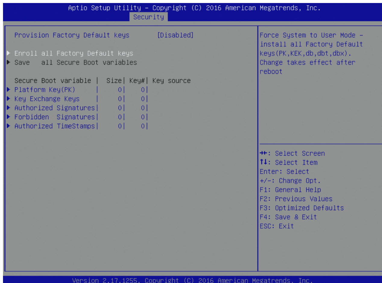
Figure 113: Key Management Menu Screen
