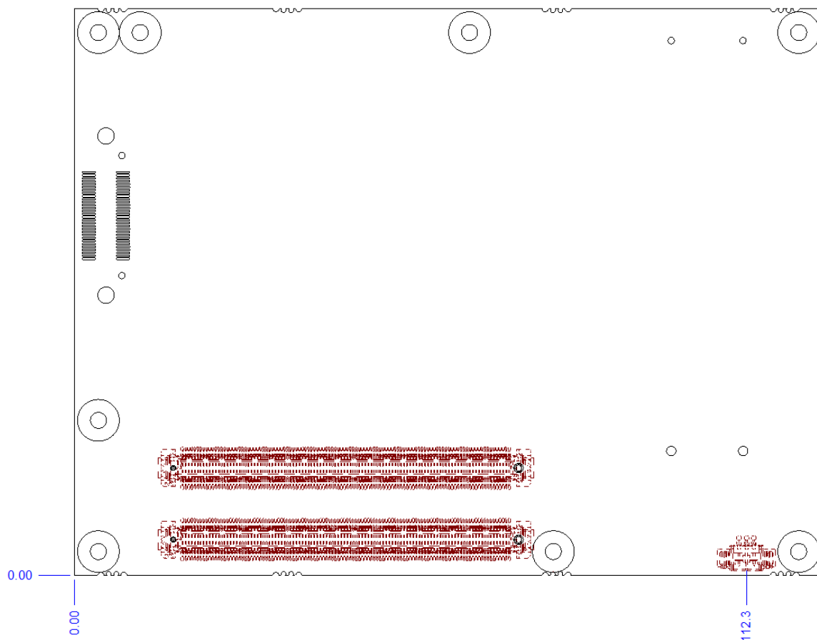
Figure 7: Location of the FAN Connectors
