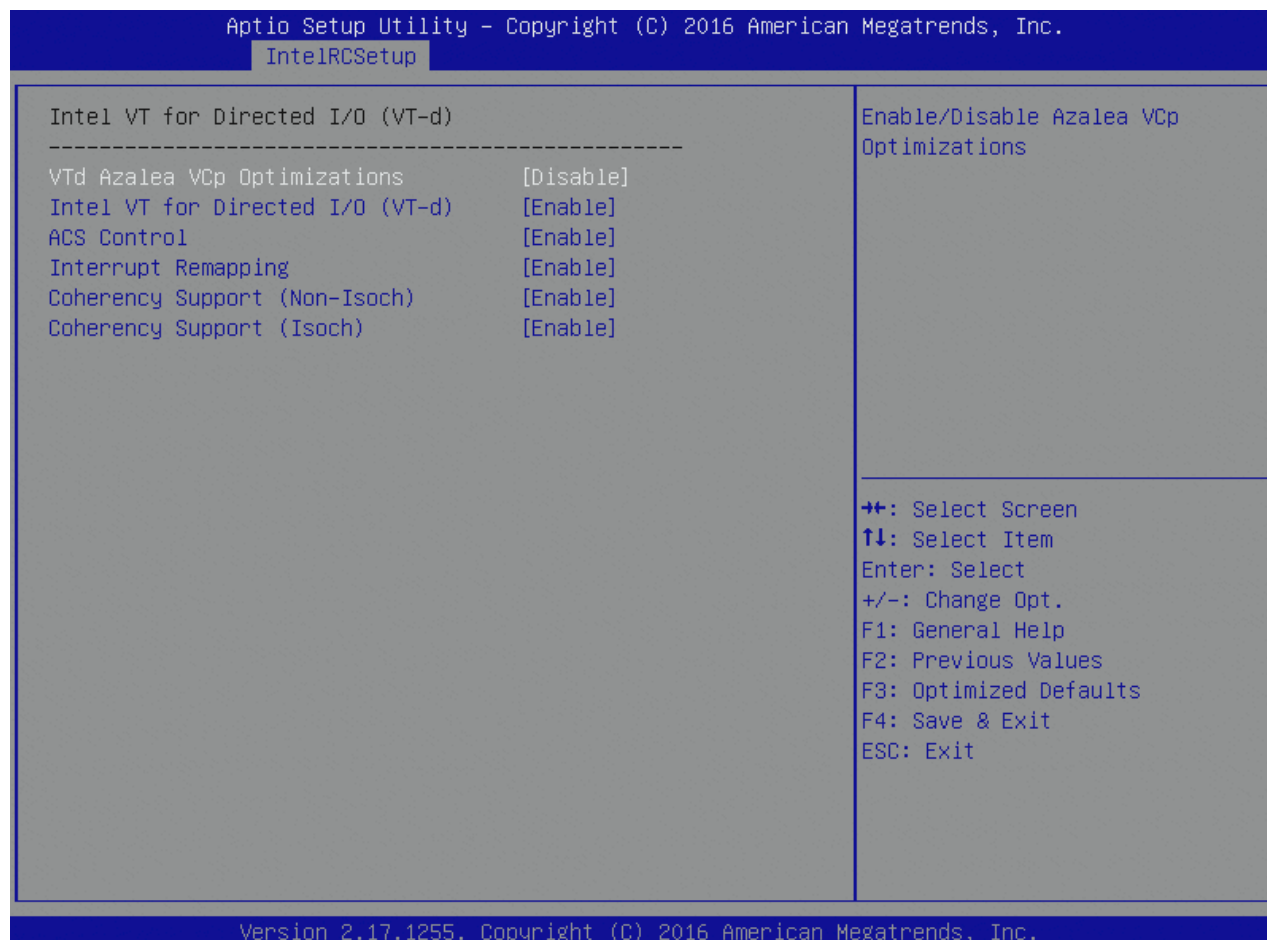
Figure 85: Intel VT for Directed I/O (VT-d) Menu Screen
