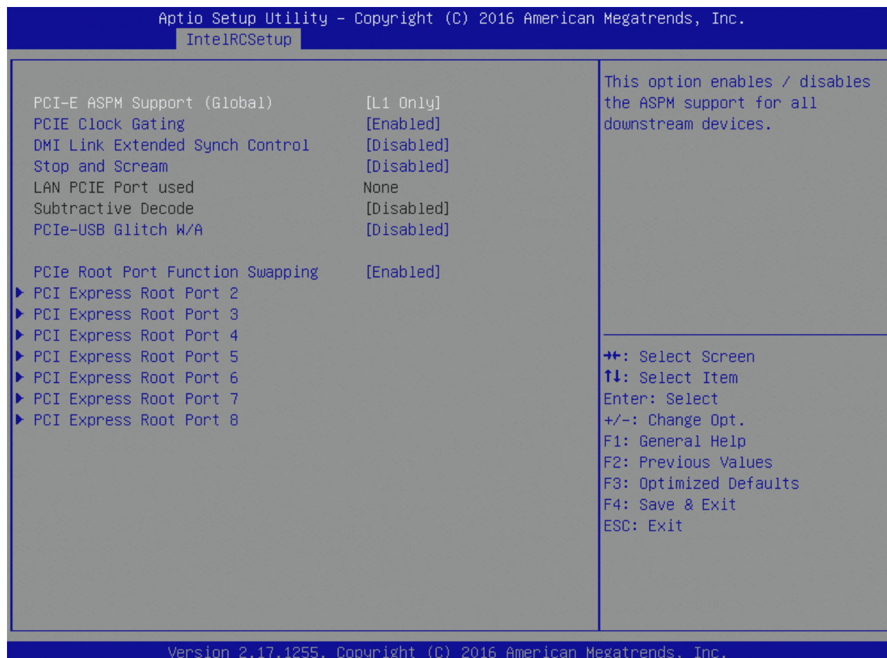
Figure 89: PCH Express Configuration Menu Screen
