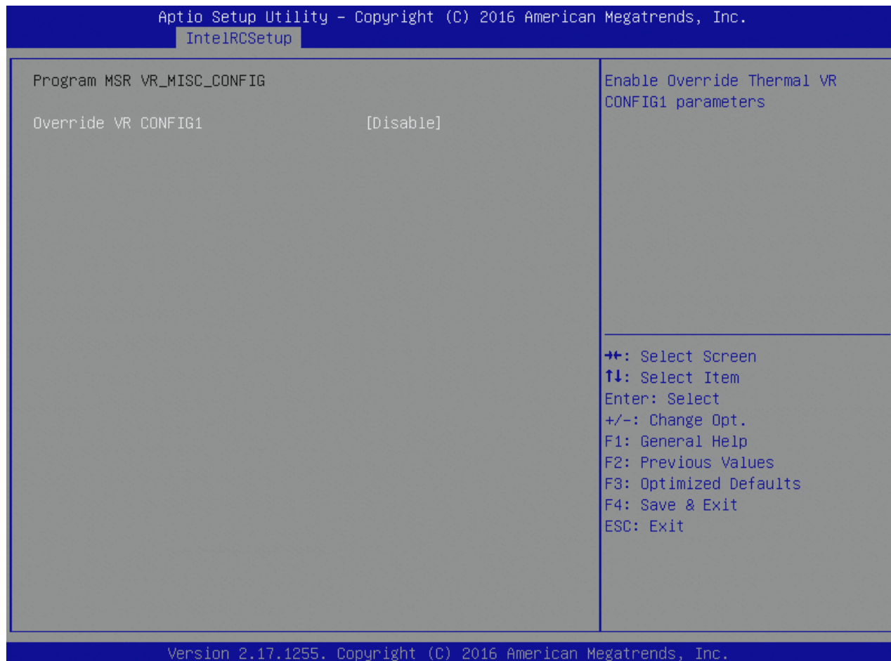
Figure 62: Program MSR VR_MISC_CONFIG Menu Screen
