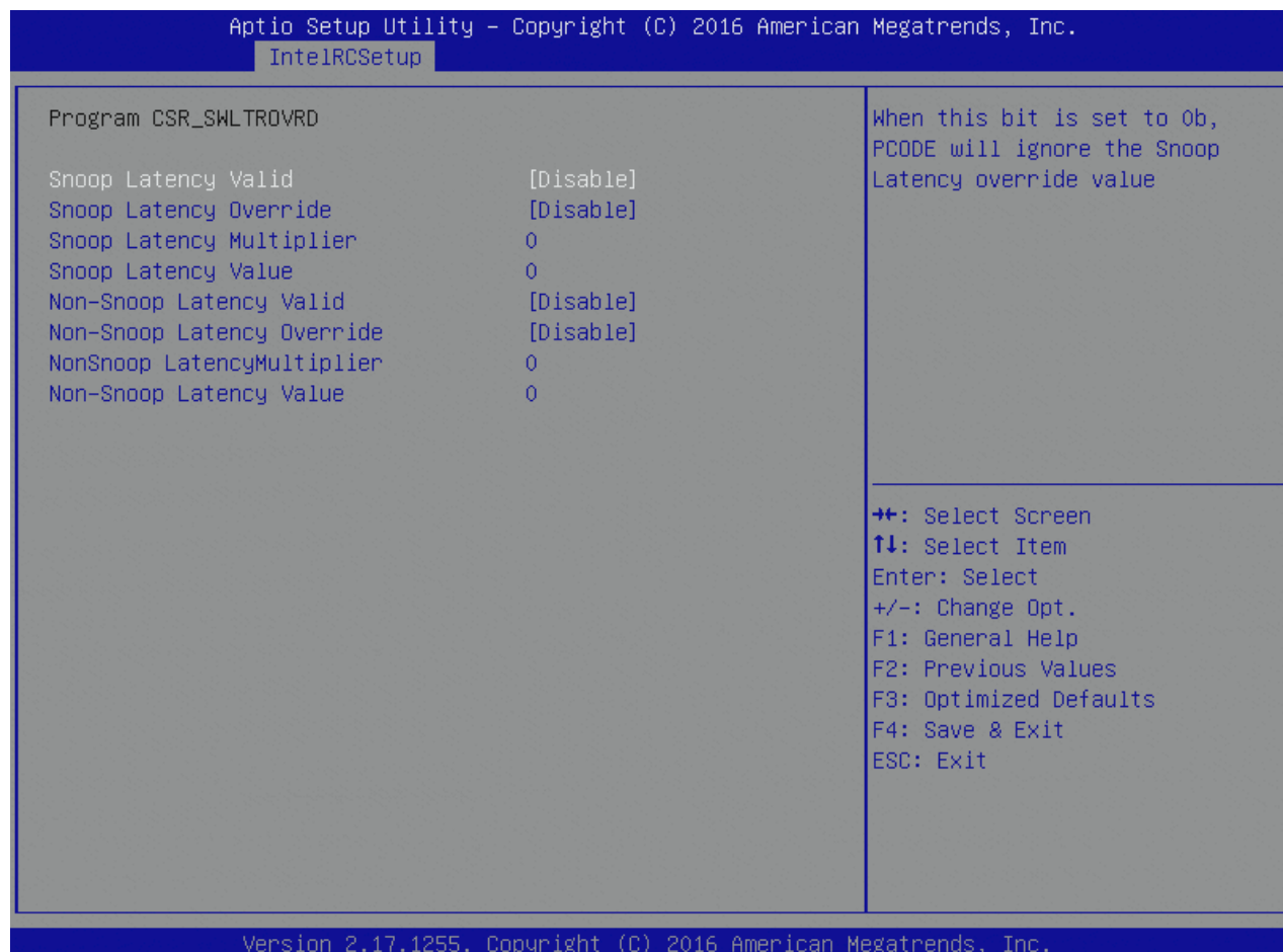
Figure 61: Program CSR_SWLTROVRD Menu Screen
