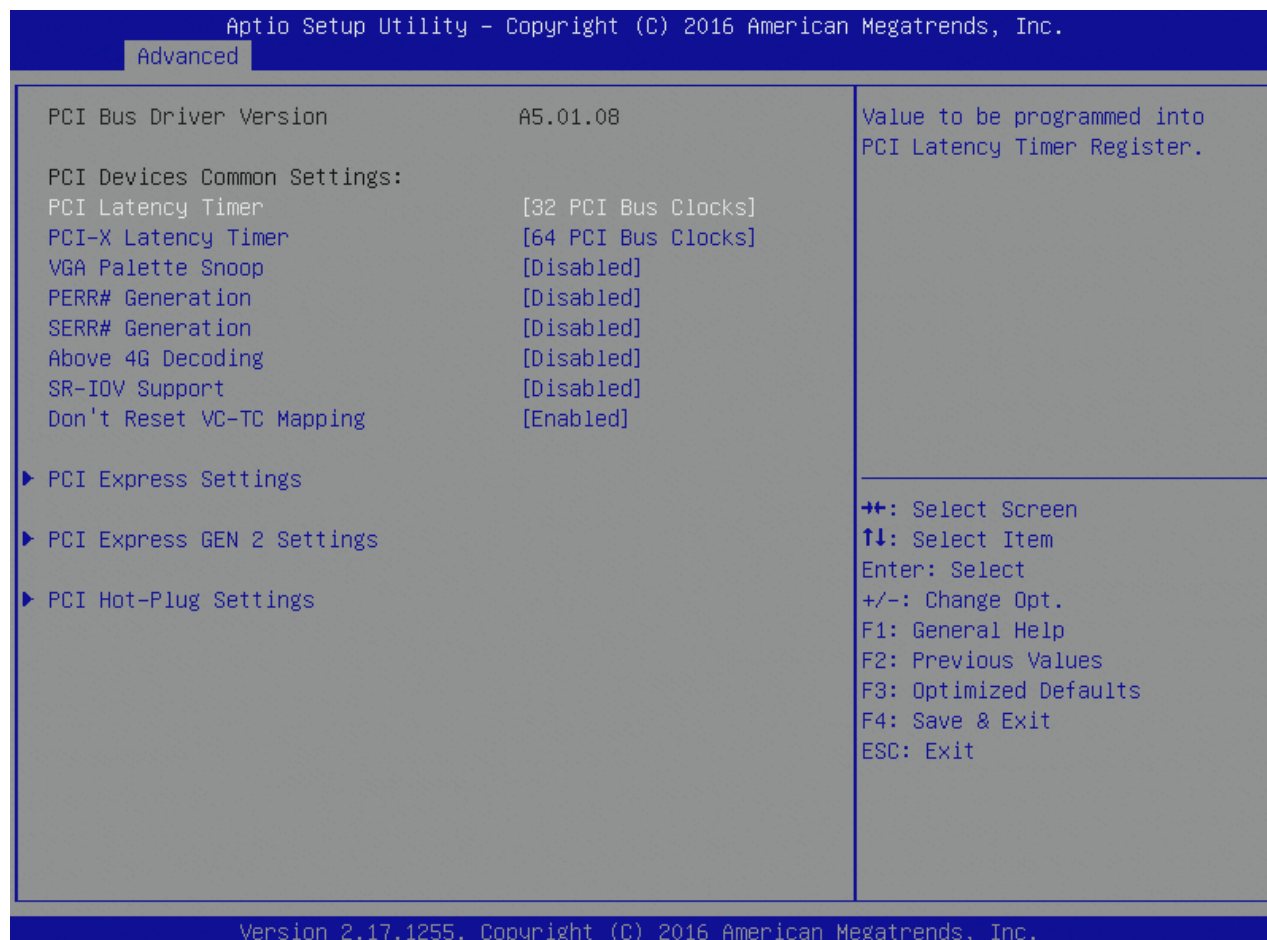
Figure 35: PCI Subsystem Settings Menu Screen
