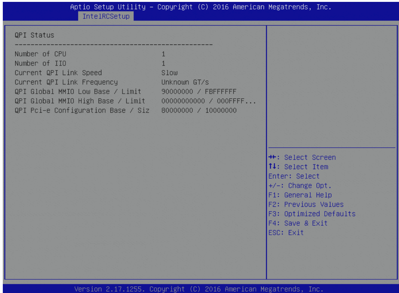
Figure 69: QPI Status Menu Screen
