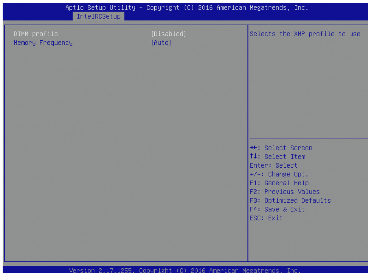
Figure 76: Memory Timings & Voltage Override Menu Screen
