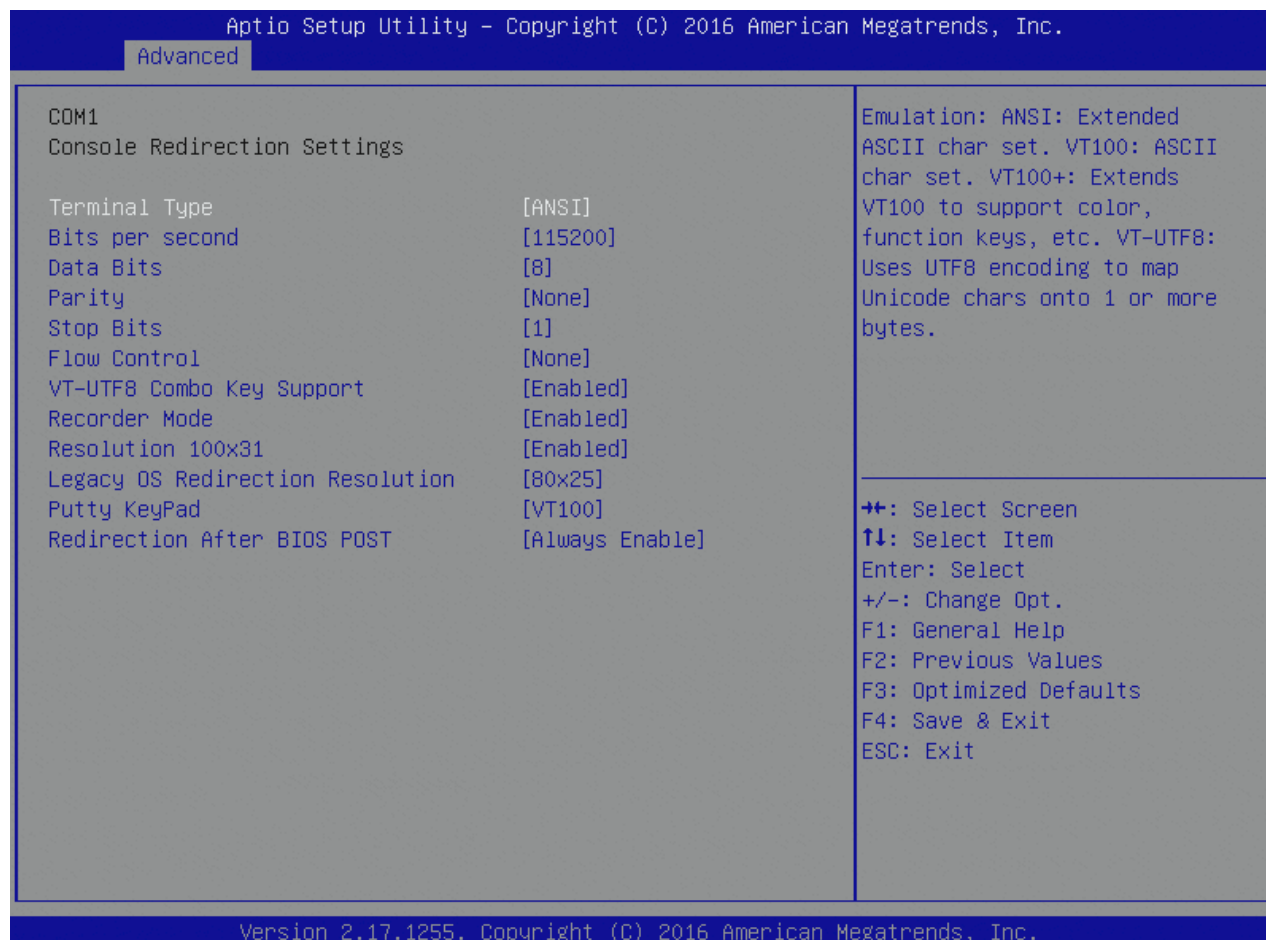
Figure 32: Console Redirection Settings Menu Screen
