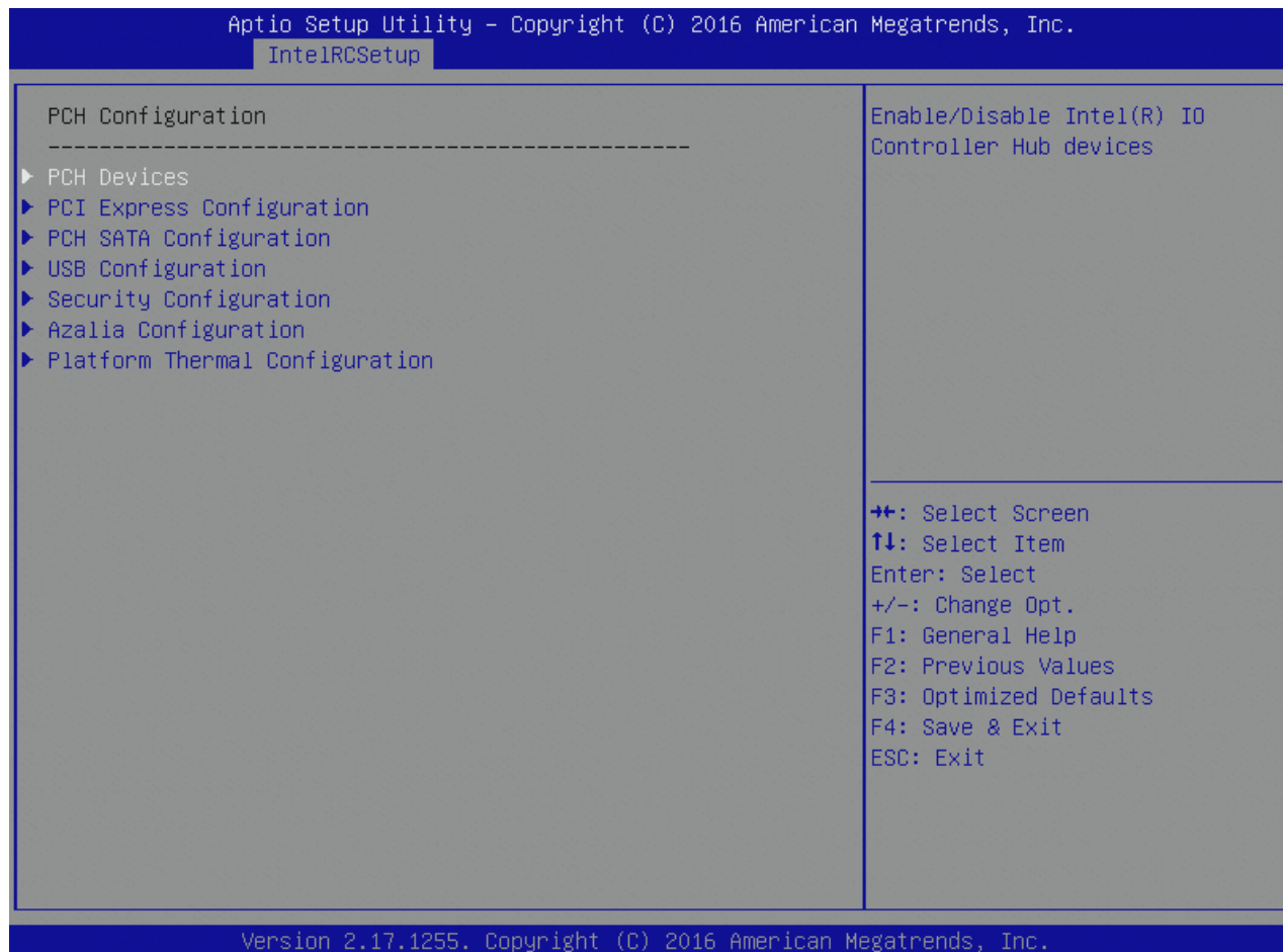
Figure 87: PCH Configuration Menu Screen
