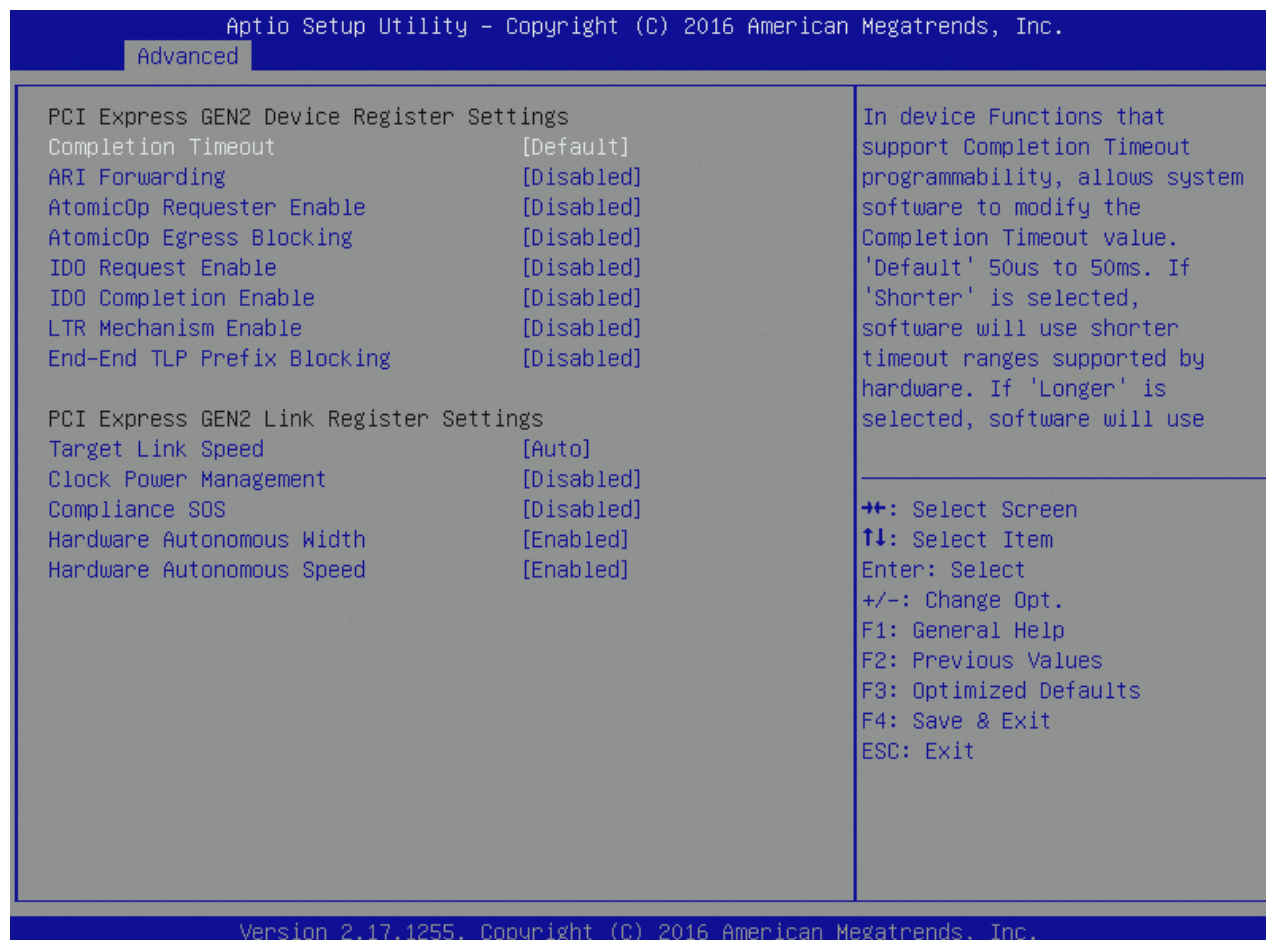
Figure 37: PCI Express Gen 2 Settings Menu Screen
