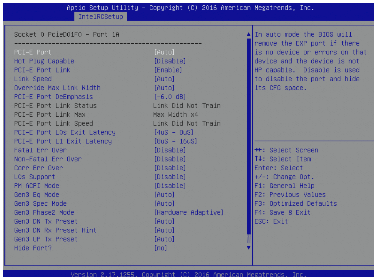
Figure 82: Socket 0 PcieD0XFX – Port XX Menu Screen
