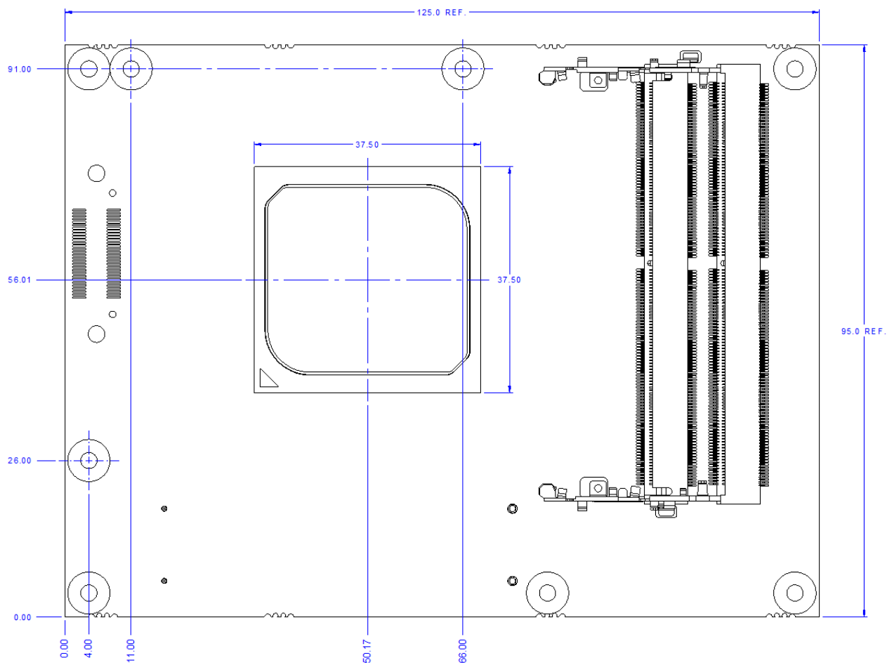
Figure 5: Module Dimensions
