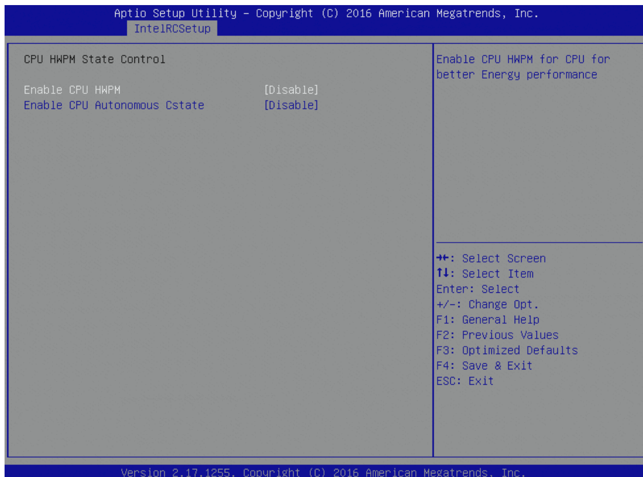
Figure 50: CPU HWPM State Control Menu Screen
