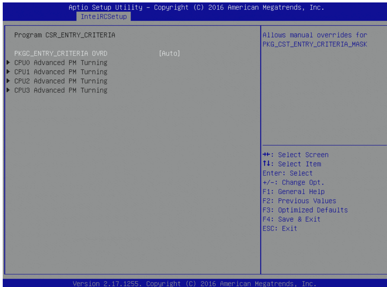
Figure 59: Program CSR_ENTRY_CRITERIA Menu Screen
