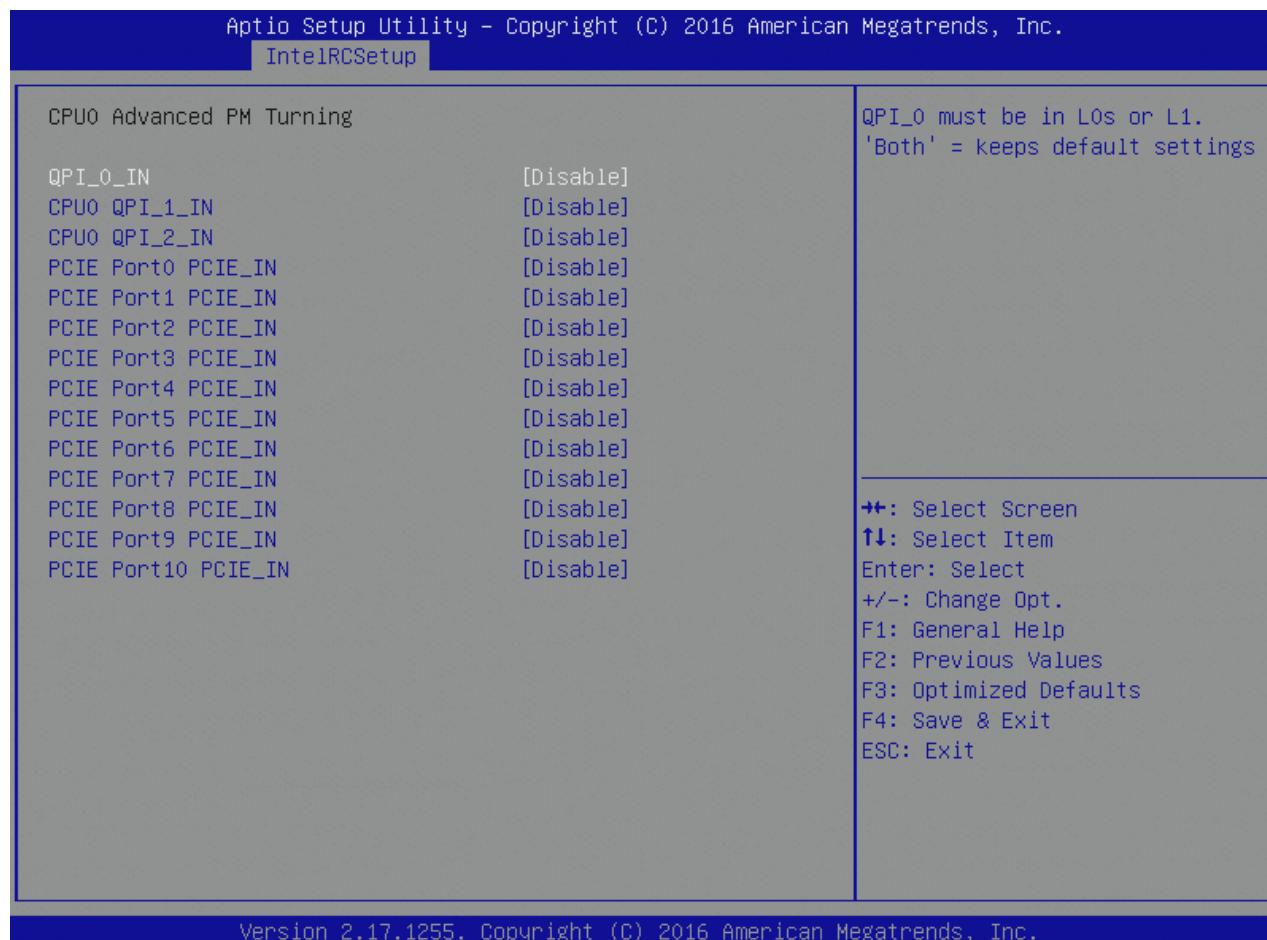
Figure 60: CPU Advanced PM Turning Menu Screen
