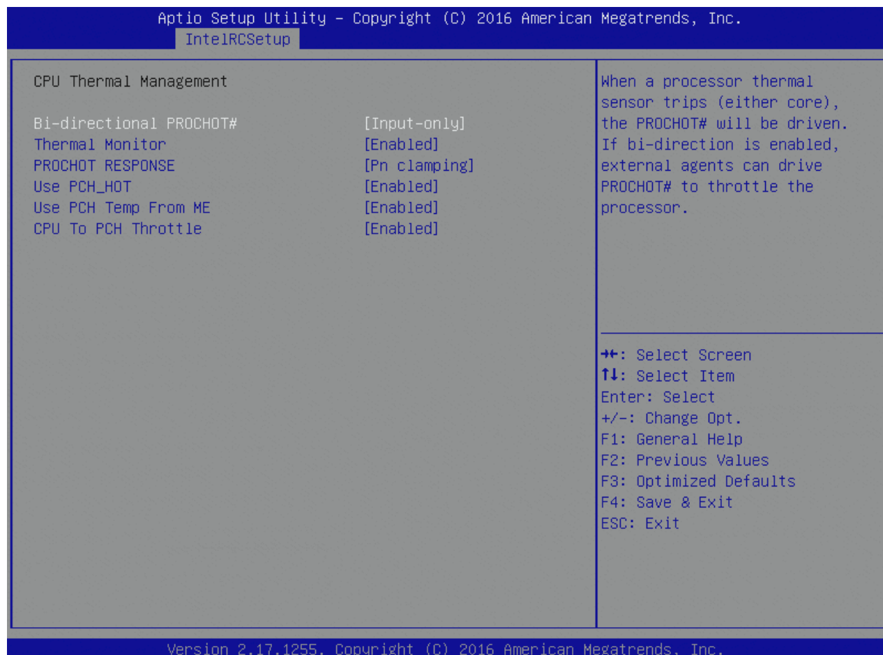
Figure 53: CPU Thermal Management Menu Screen
