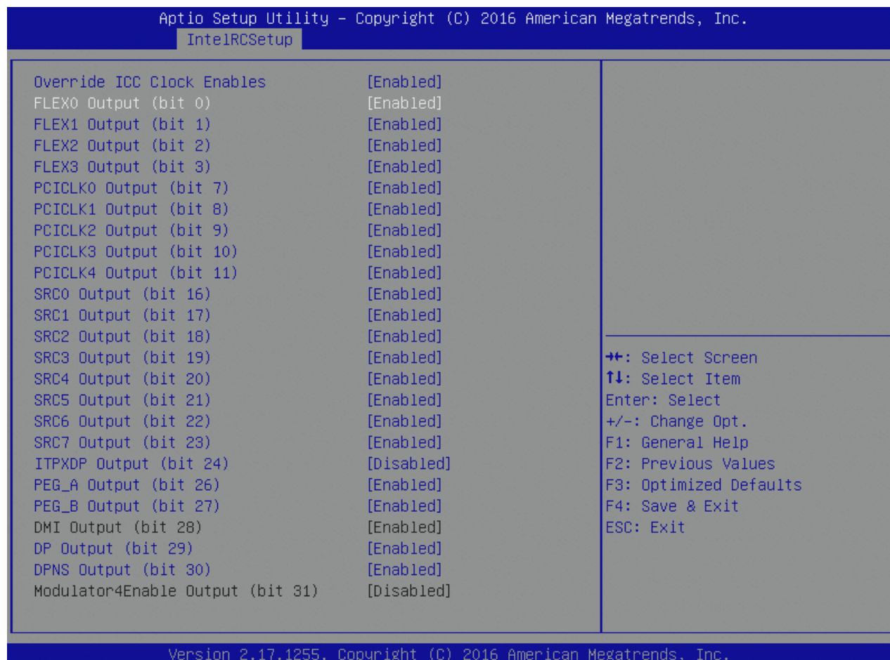
Figure 100: Override ICC Clock Enables Menu Screen
