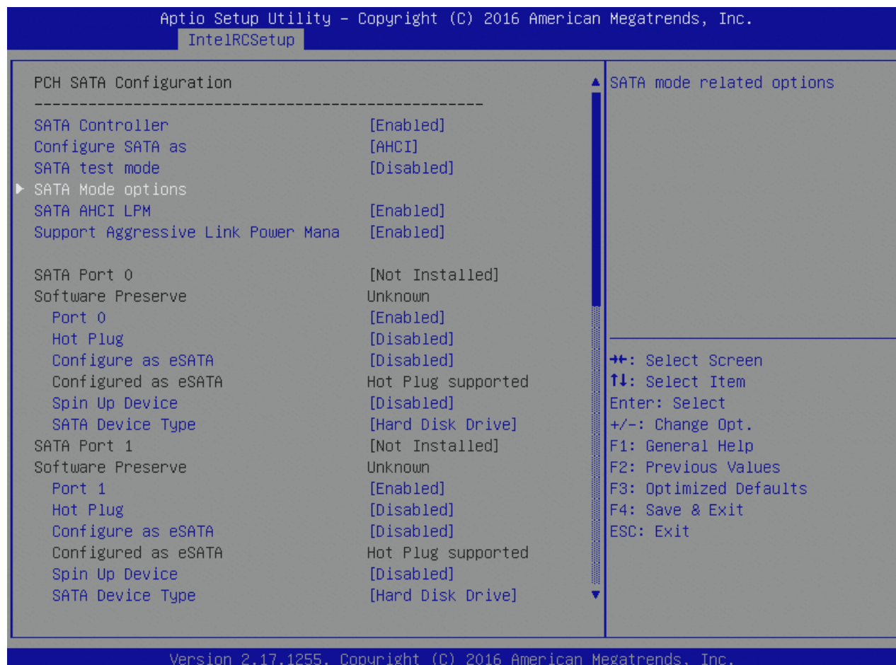
Figure 91: PCH SATA Configuration Menu Screen
