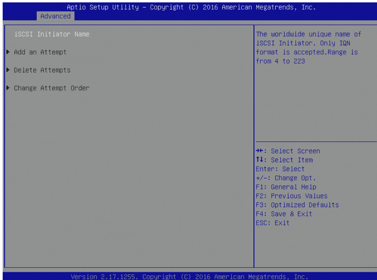
Figure 15: iSCSI Configuration Menu Screen
