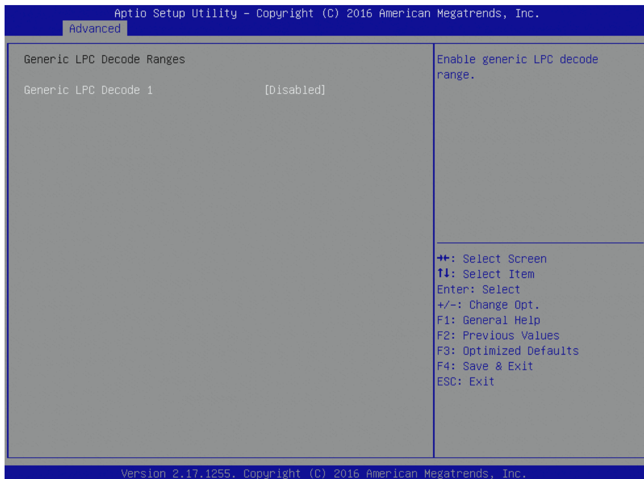
Figure 19: Generic LPC Decode Ranges Menu Screen
