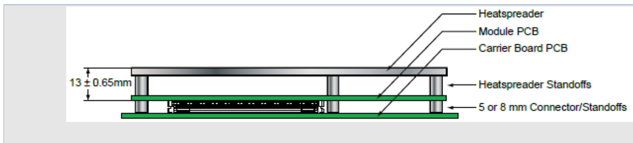
Figure 6: Module Height
