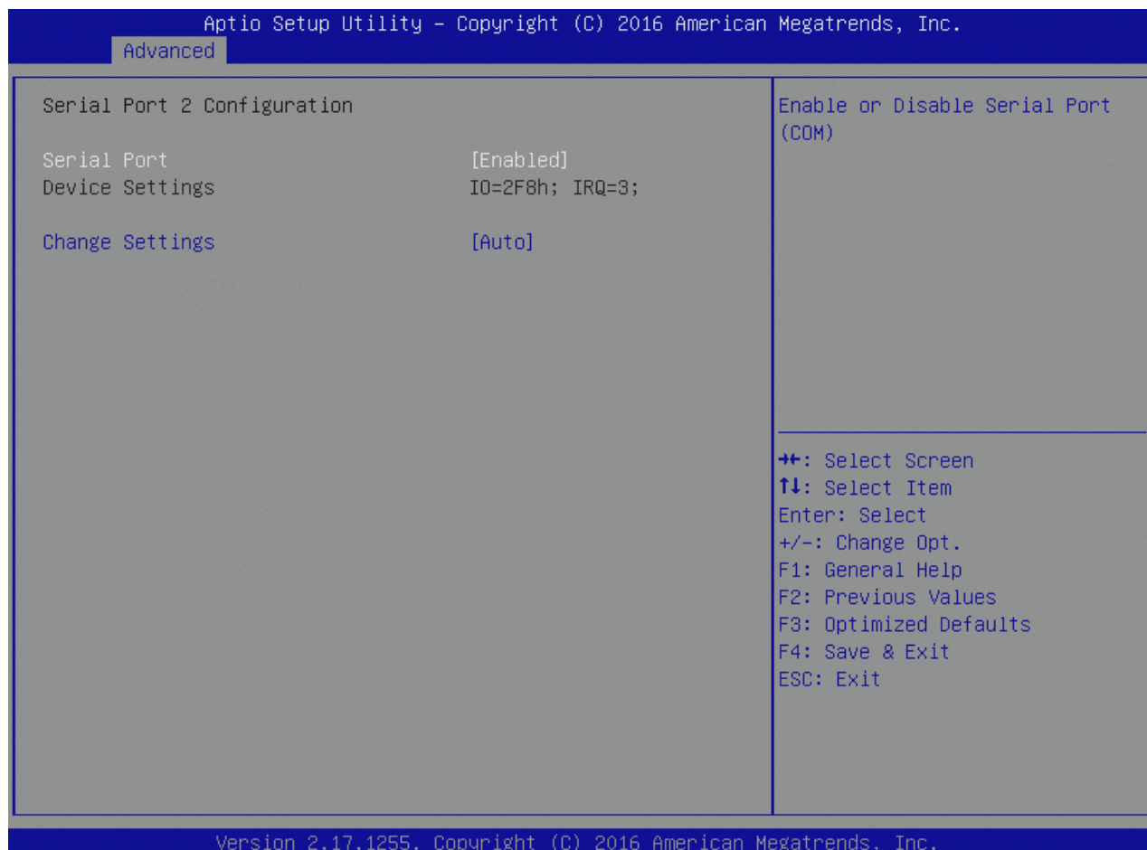
Figure 25: FPD UART Serial Port 2 Configuration Menu Screen
