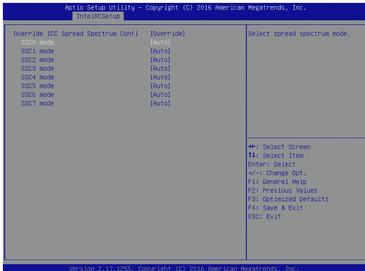
Figure 101: Override ICC Spectrum Configuration Menu Screen
