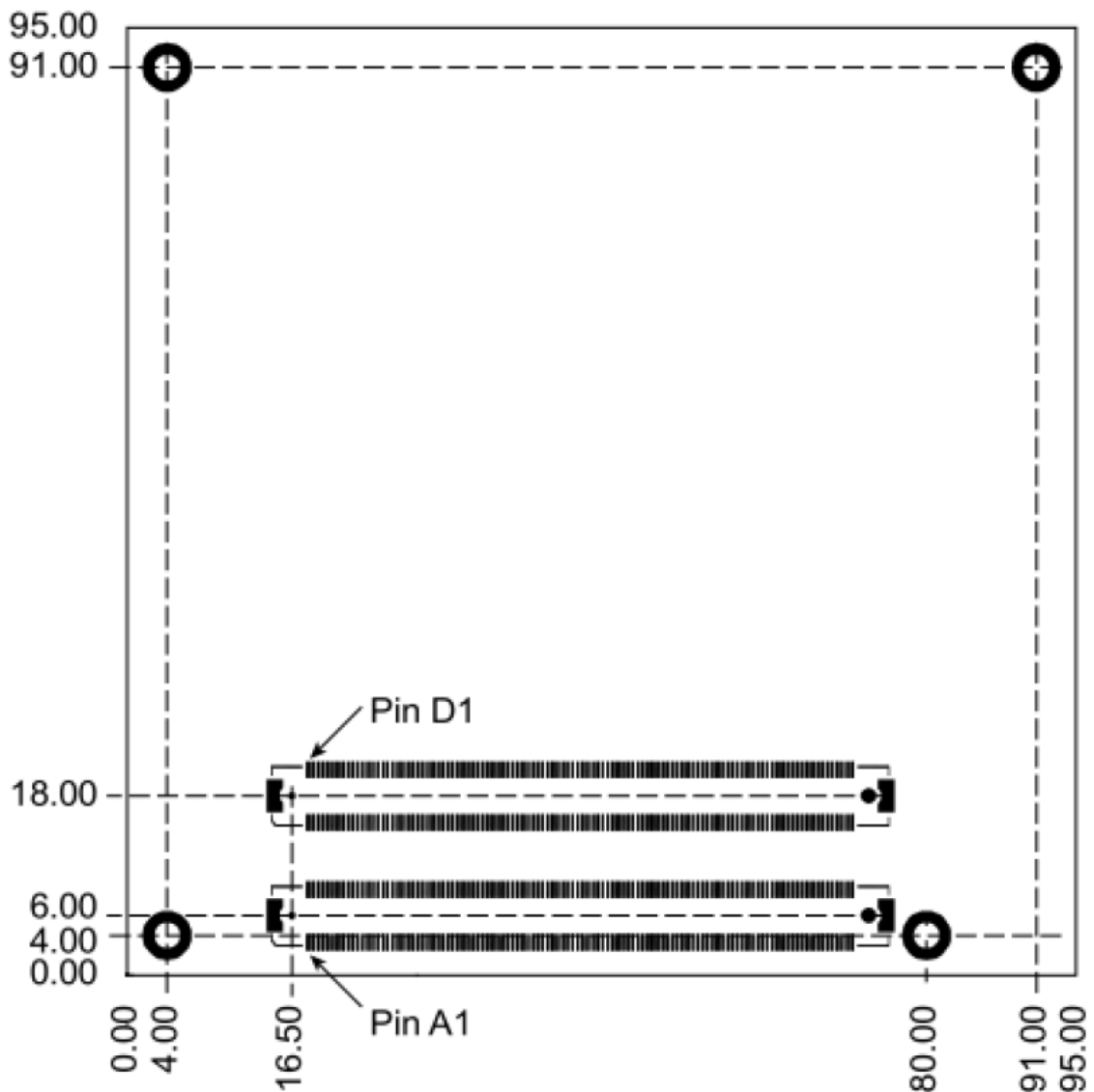
Figure 3: Module Dimensions
