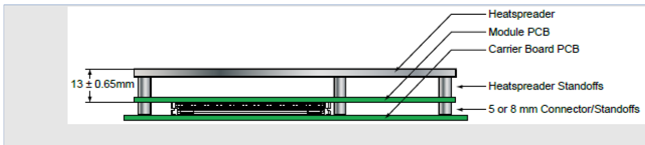
Figure 4: Module Height
